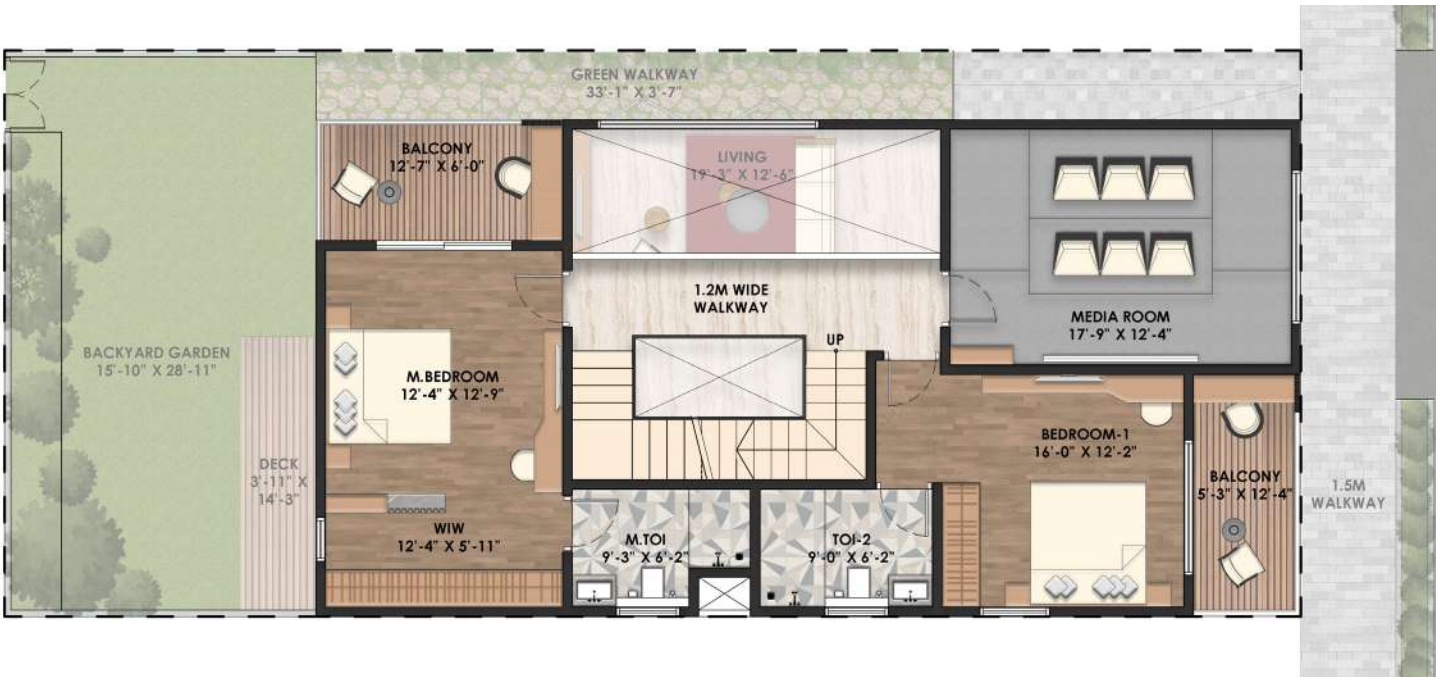
FIRST FLOOR
