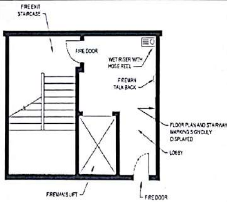
(LAYOUT TO BE PLANNED AS PER PROJECT BASIS MEETING ALL THE REQUIRED DETAILS)
